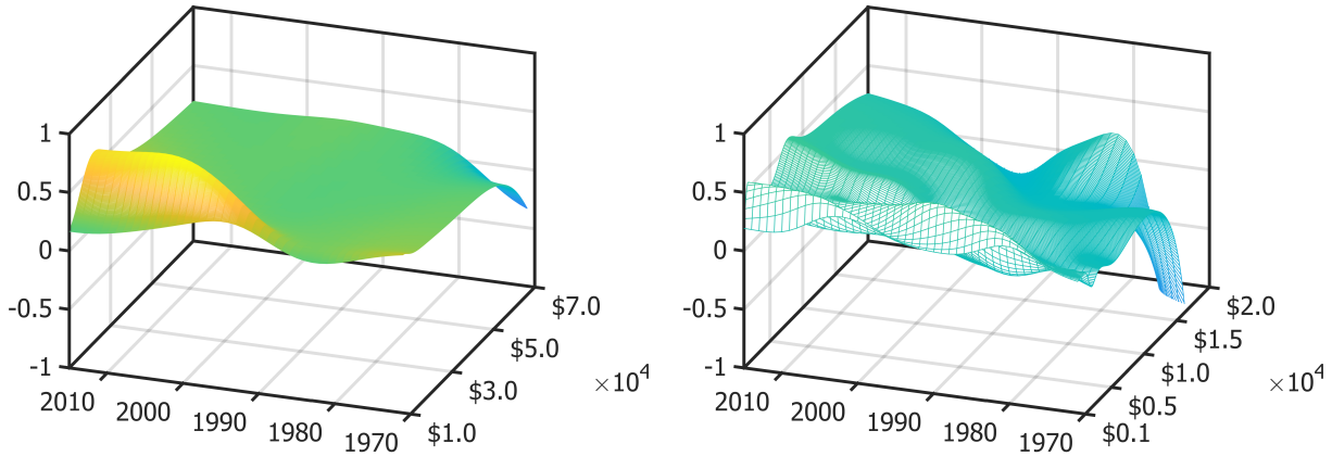
Figure 3: Estimated Elasticity Surfaces. Estimates of the common components \Phi(r, x) = \Gamma(r, x) + \Gamma_x(r, x)x of the energy-GDP elasticities for the energy intensity-reducing group (left) and the energy intensity-increasing group (right). The surfaces are bias-corrected using the bootstrap procedure described in Appendix C.
