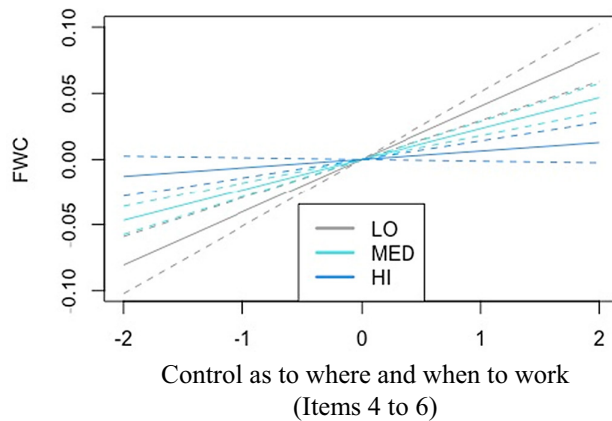
FIGURE 5 Conditional indirect effect of control as to where and when to work (items 4–6) via supplemental work and work-to-family conflict at low, medium and high values moderator segmentation norms (dotted lines are confidence intervals).
