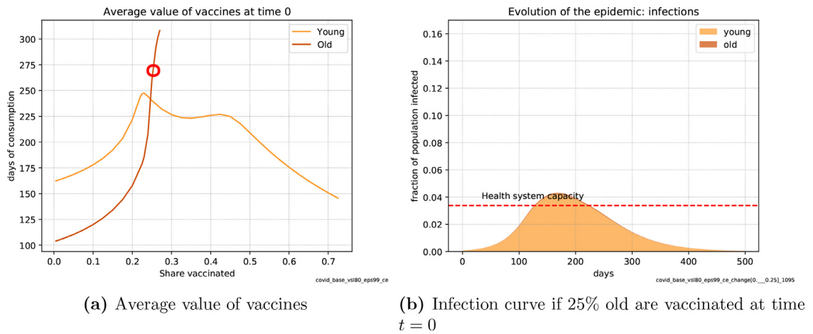
Fig. 6. The average value of vaccinating 25% of the population, all old, and the infection curve associated with such an intervention.
