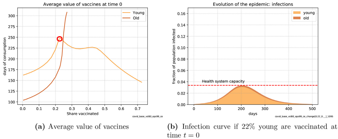
Fig. 5. The average value of vaccinating 22% of the population, all young, and the infection curve associated with such an intervention.
