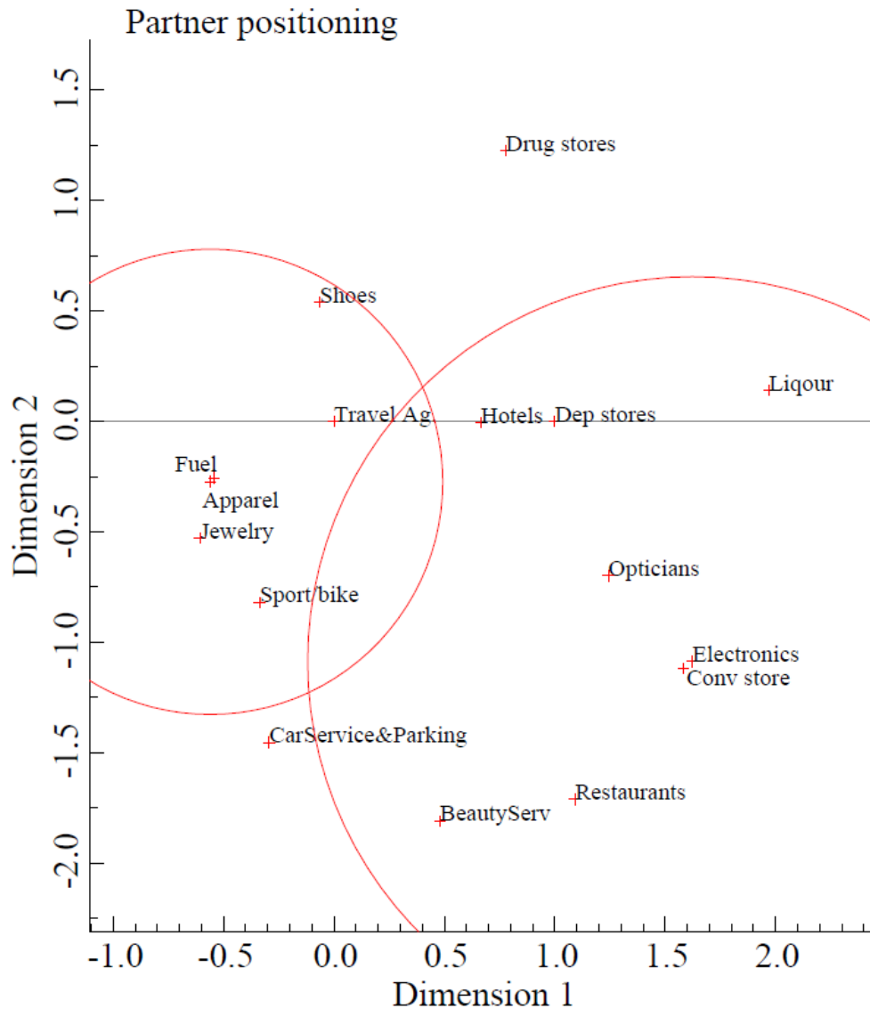
Figure 3: Graphical representation of cross-partner weights
