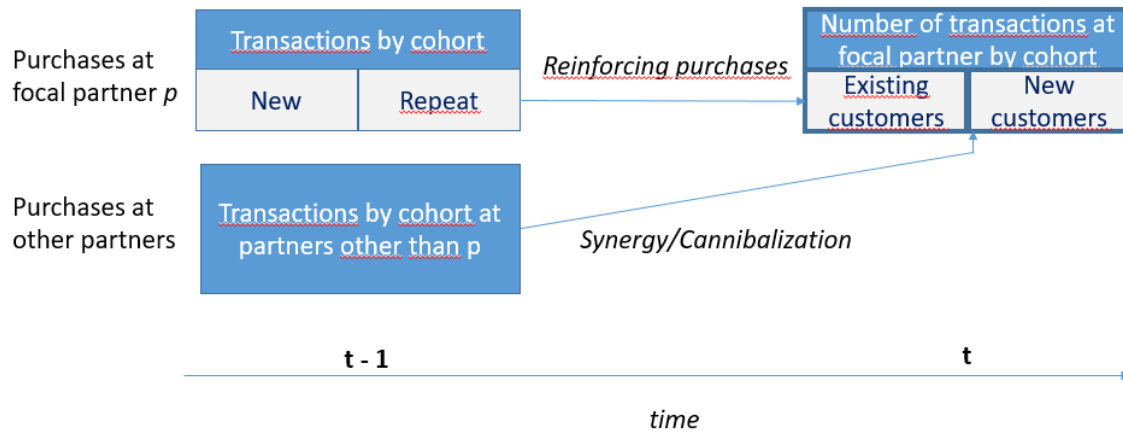
Figure 2: Graphical representation of the modeling approach
