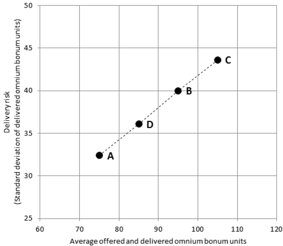
Fig. 2. An essential idea of the experimental design: the more omnium bonum is offered (and delivered) on average, the greater the risk of delivery, as measured by the standard deviation
