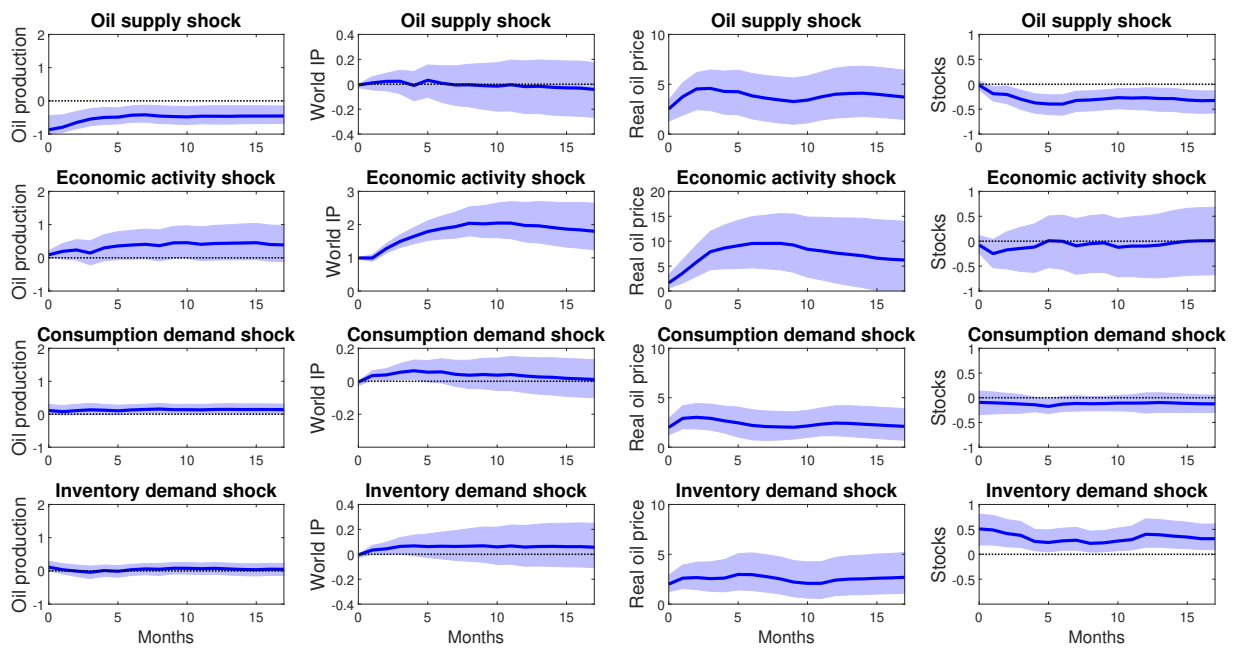
Figure A5: Structural impulse response functions: oil market variables
