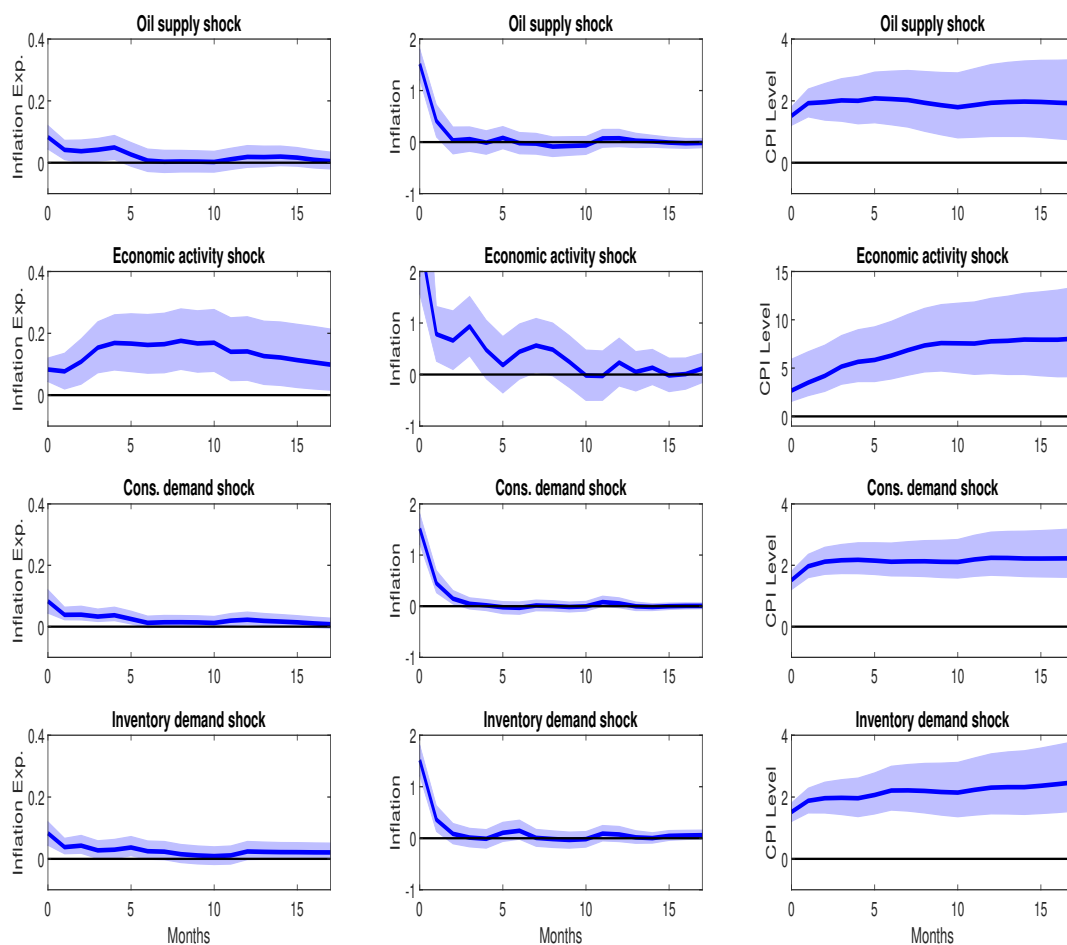
Figure 2: Structural impulse response functions
