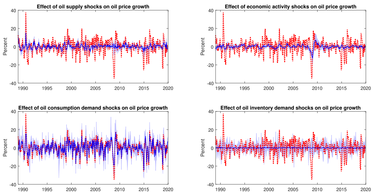
Figure A6: Structural historical decompositions: oil market variables
