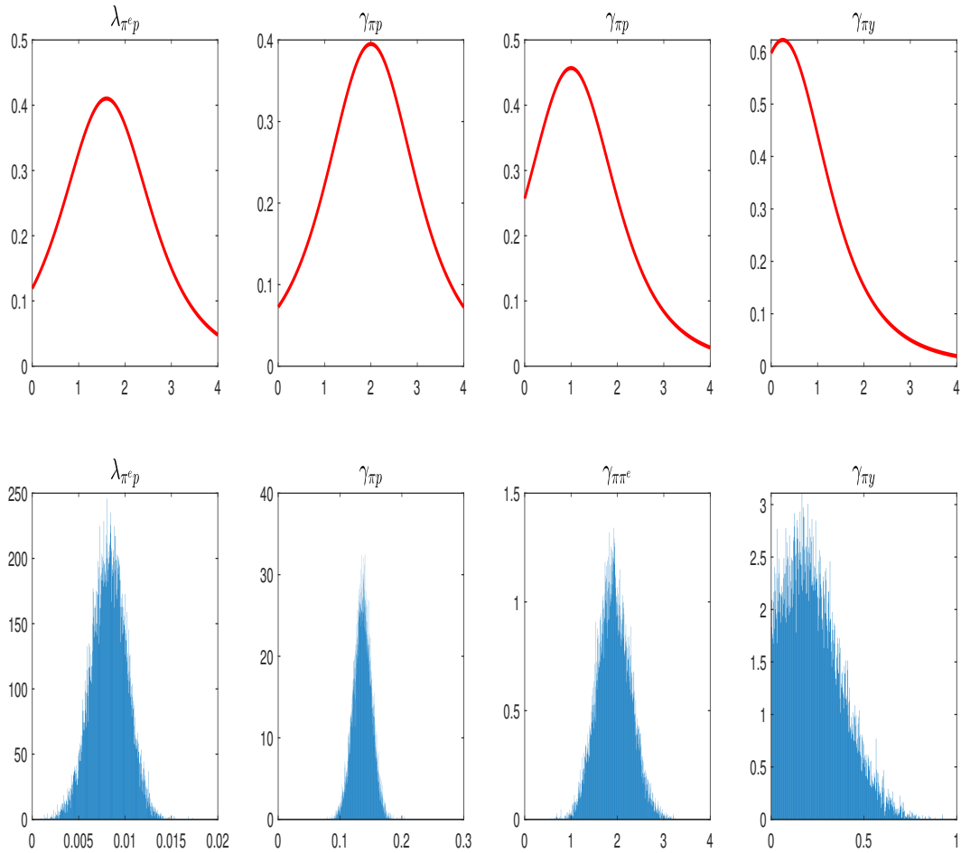
Figure 1: Prior (solid red curves) and posterior (blue histograms) distributions of structural parameters in the inflation block
