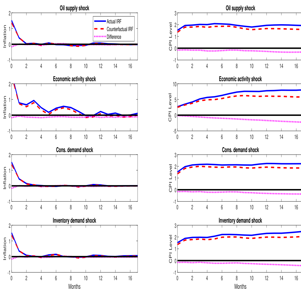
Figure 4: Actual (blue solid line) and counterfactual (red dashed line) structural impulse response functions and their difference (magenta dotted line)
