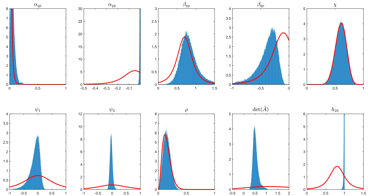
Figure A4: Prior (solid red curves) and posterior (blue histograms) distributions of structural parameters in the oil block
