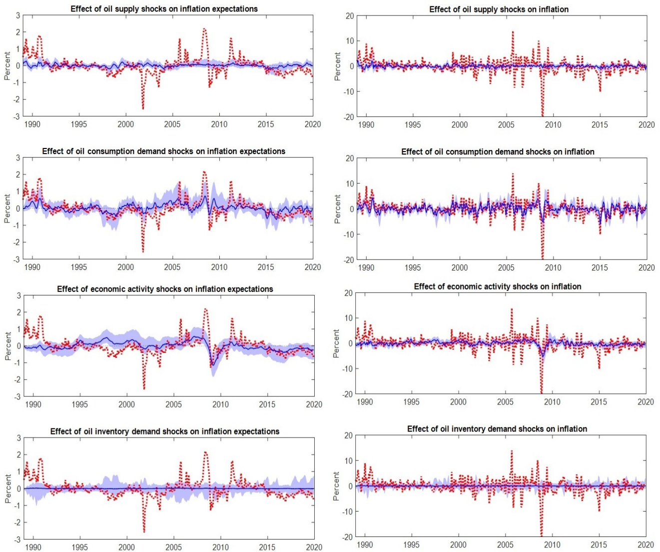
Figure 3: Historical Decompositions: Expected and realized inflation
