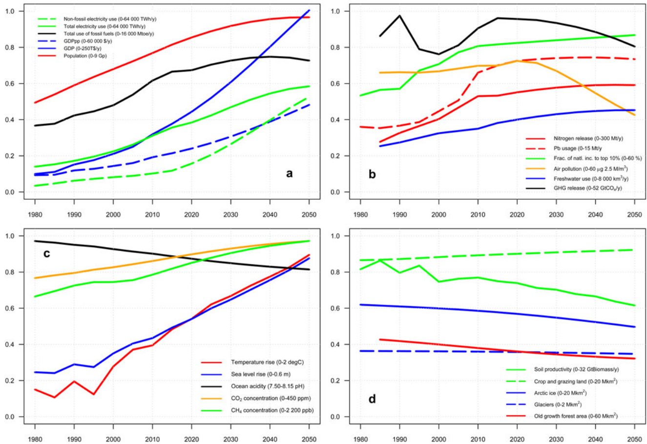
Fig. 3. Outputs from the socio-economic sub-model Earth3-core (a and b) and the biophysical model ESCIMO-plus (c and d) used to drive the Performance sub-model. Details in Goluke et al. (2018). All outputs scaled from 0–1; output scale range given in key below each panel.
