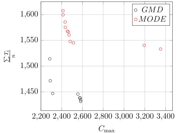
Fig. 5. Comparison of GMD and MODE using the instance dpp02a .
