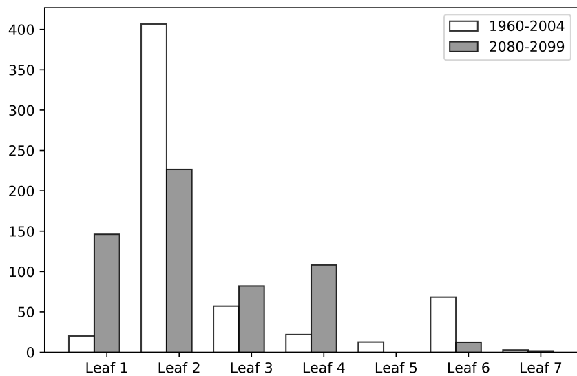
Figure 5: Average annual distribution of state-month observations across the leaves defined by the regression tree (see figure 3) for the periods 1960-2004 and 2080-2099.
